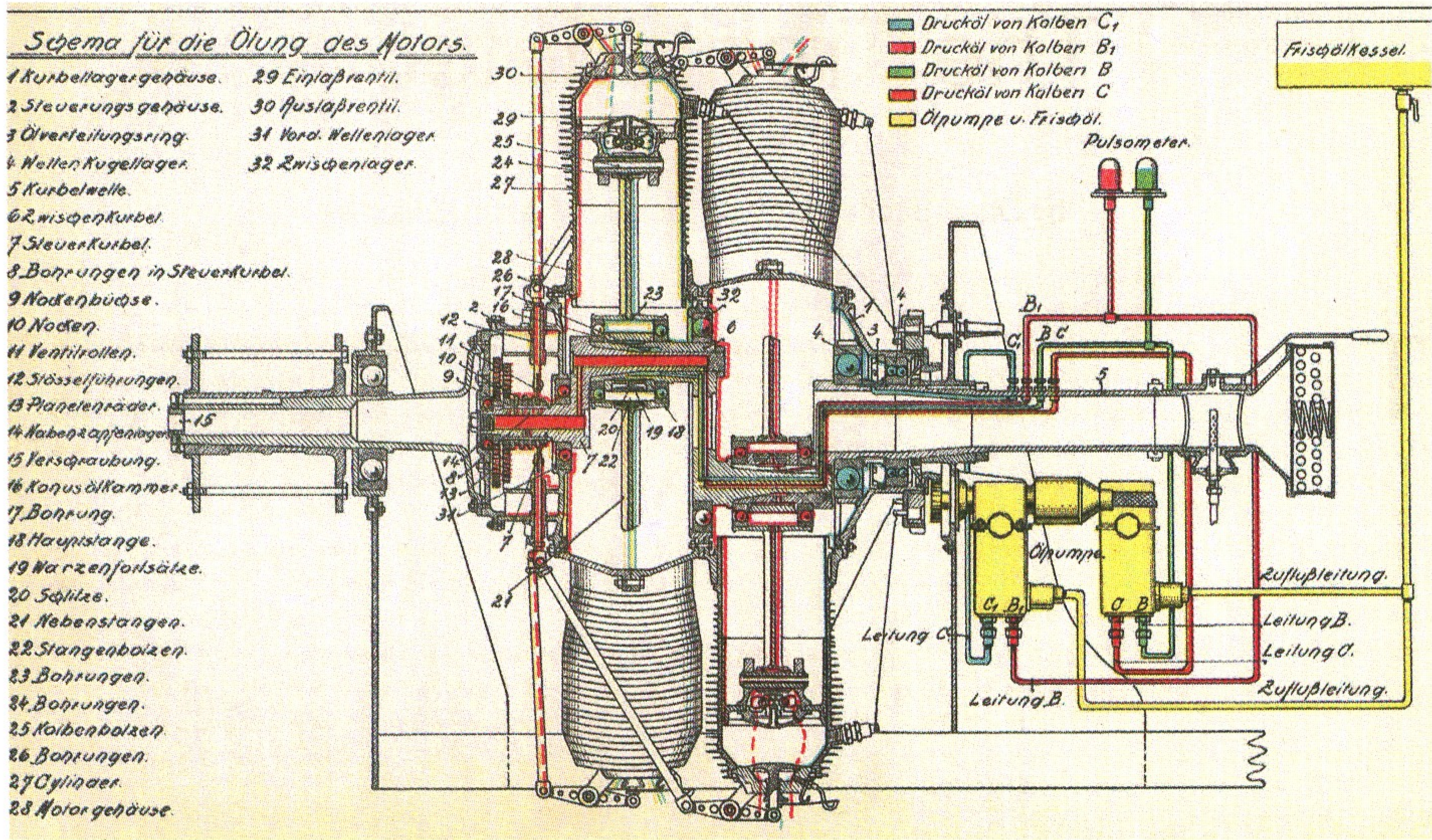
Oberurseler 160PS Umlaufmotor U III – lubrication scheme with inlet valve arrangement
